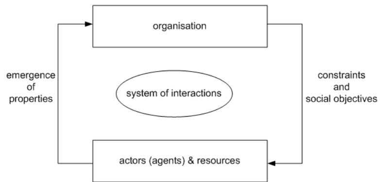
Figure 1: Self-organising system
