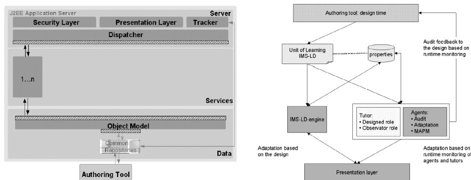
Figure 3 The aLFanet framework: (left) the technical architecture (Carrion et al., 2004) (right) ‘IMS LD as communicator’ in between the various services
