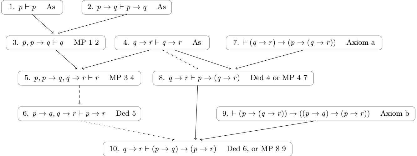
Figure 2: A DAM for the proof of q \rightarrow r \vdash (p \rightarrow q) \rightarrow (p \rightarrow r)
