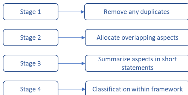
Figure 3, synthesis process
