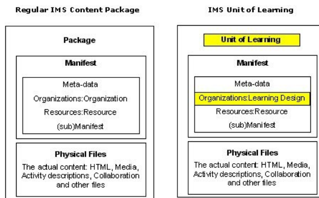
Figure 5. In IMS LD the organization element of a regular IMS Content Package is replaced with the Learning Design elements
