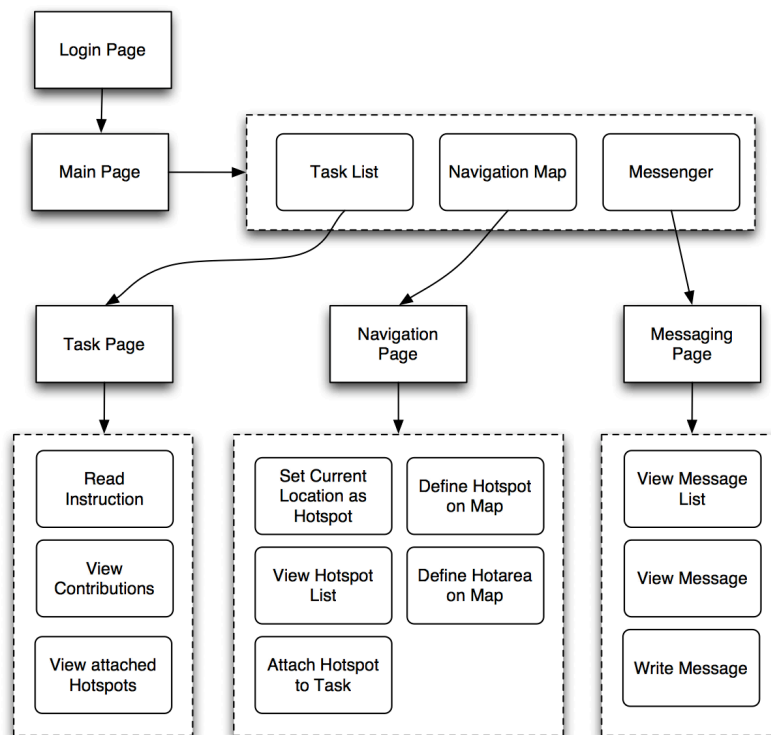
Fig. 2. The information architecture of the scouting application.
